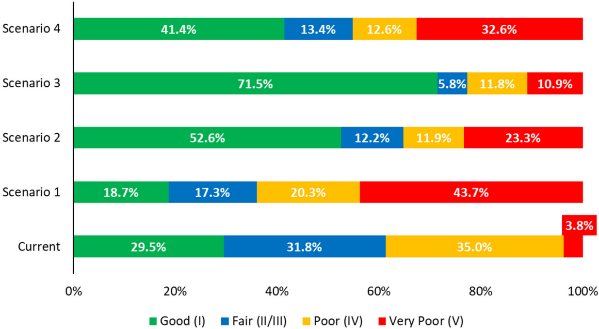
Figure 14. Comparison of Pavement Condition by FY 34/35 by Scenarios.
