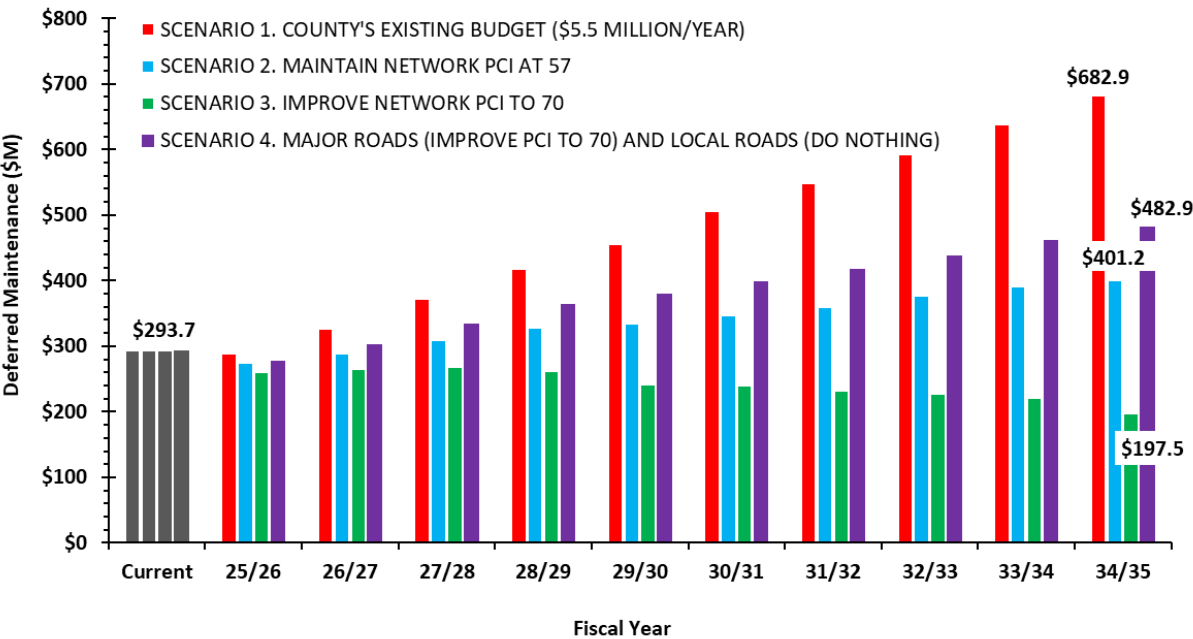
Figure 13. Comparison of Annual Deferred Maintenance by Scenario.
