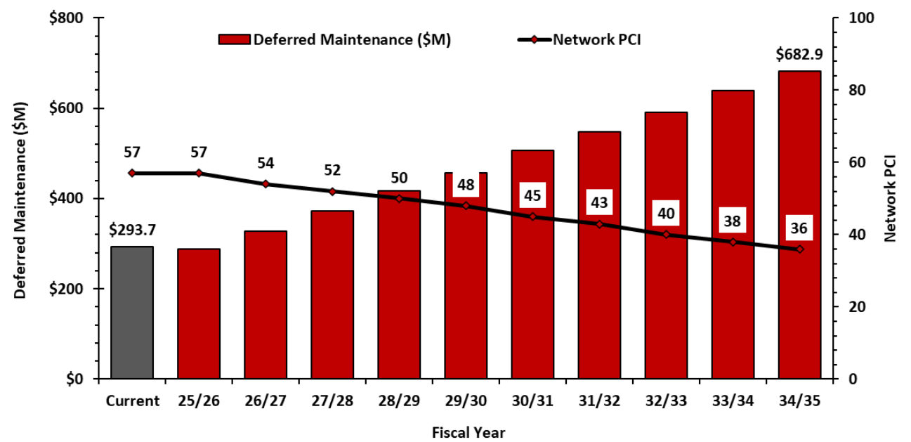
Figure 8. PCI versus Deferred Maintenance for Scenario 1.
