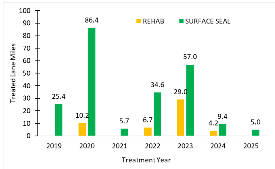
Figure 4. Treated Lane-Miles After 2018/19 PMP Update
