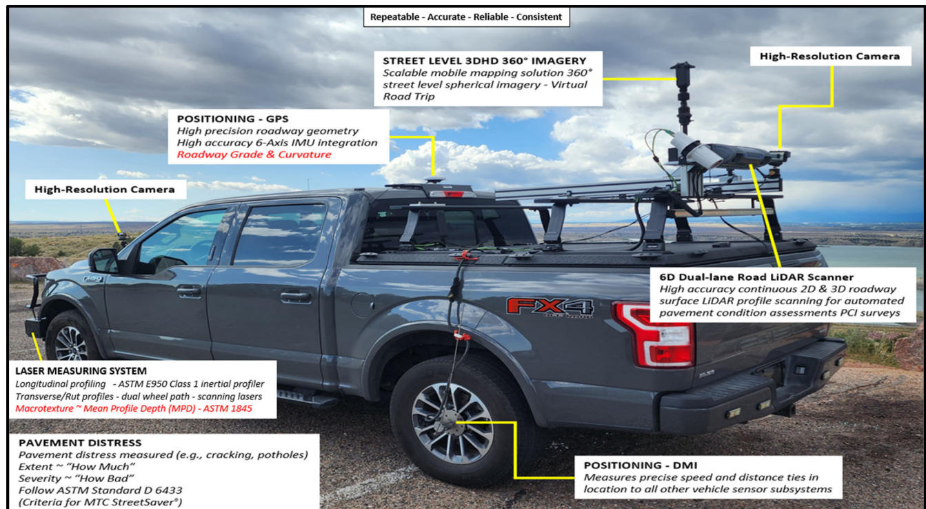
Figure 1. Roadway Collection Vehicle System.
