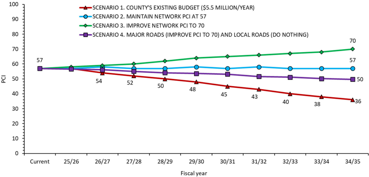
Figure 12. Comparison of Annual PCI by Scenario.
