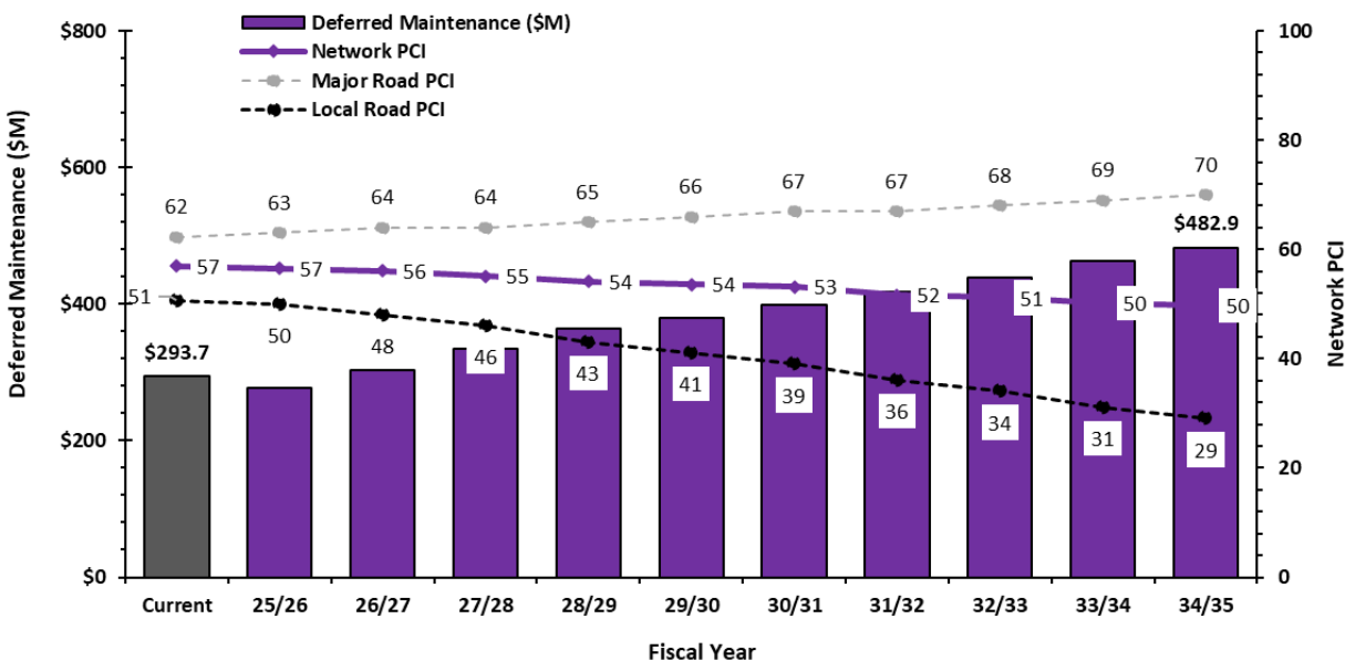
Figure 11. PCI versus Deferred Maintenance for Scenario 4.
