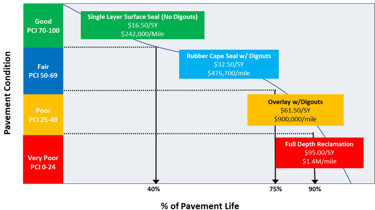
Figure 7. Costs 6 of Maintaining Arterial over Service Life.
