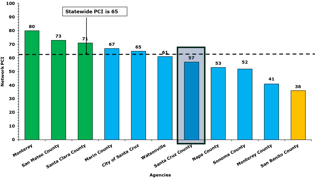
Figure 6. Network PCI for Different Agencies.
